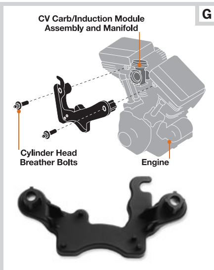
G. INDUCTION ALIGNMENT BRACKET KIT
