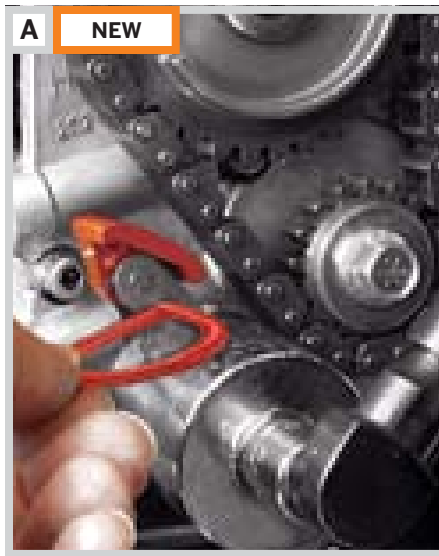
A. SCREAMIN' EAGLE TWIN CAM CHAIN TENSIONER TOOL
